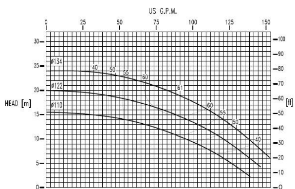
CM30 Curve
